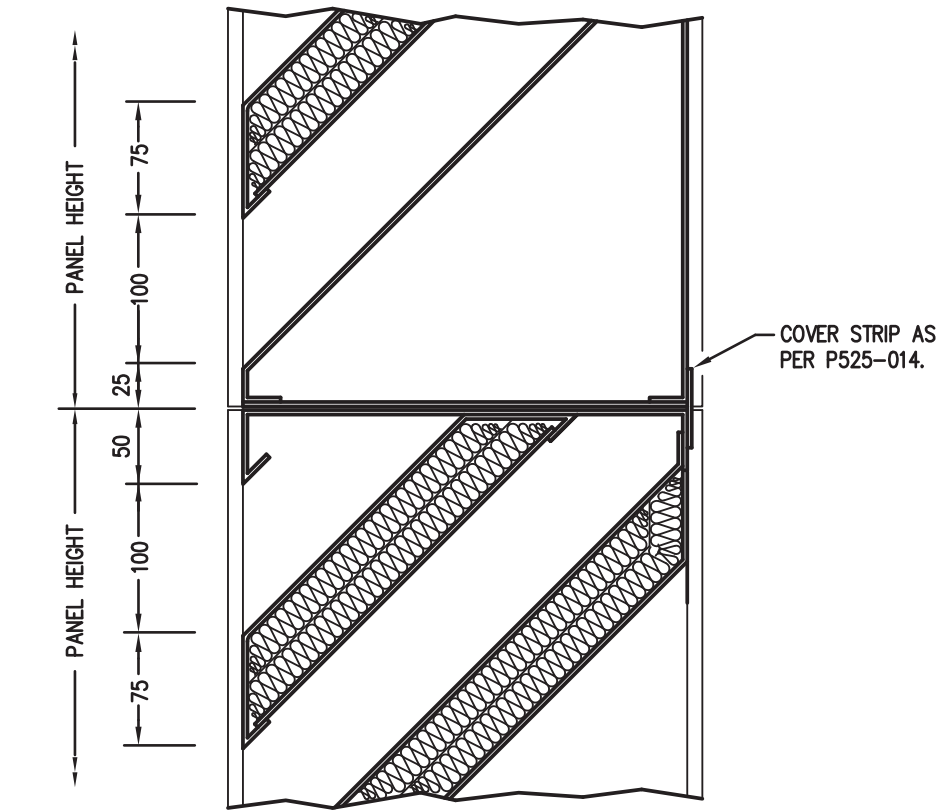
873. VERTICAL JOINT DETAIL
