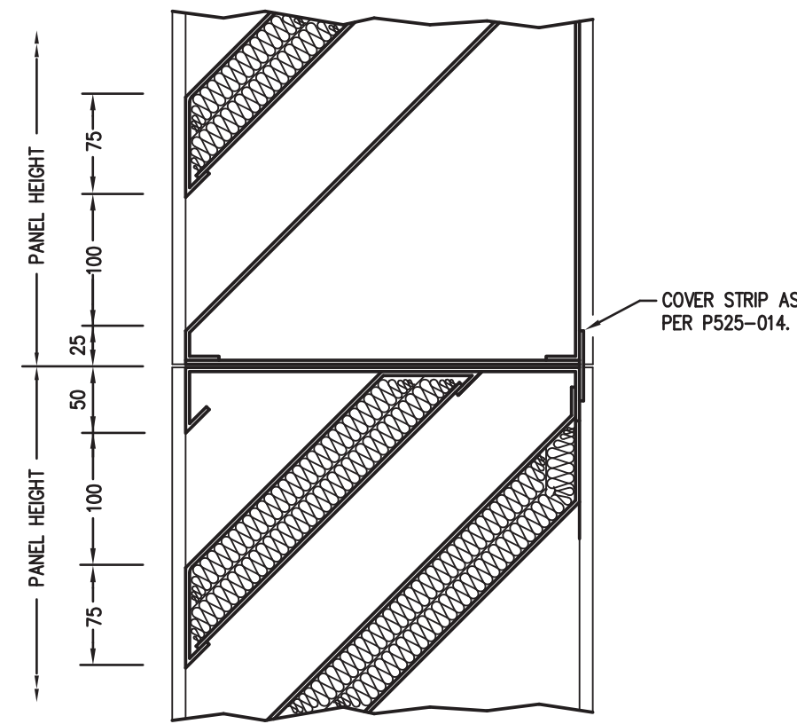
873. VERTICAL JOINT DETAIL
