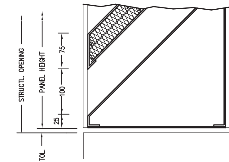
876. CILL DETAIL
