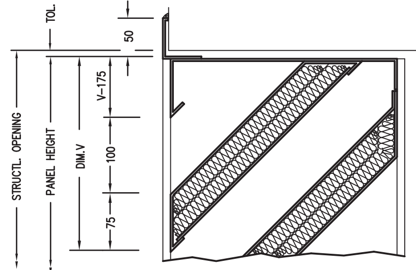
870. HEAD DETAIL
