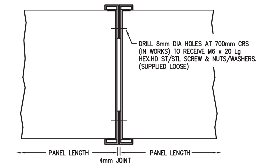
874. HORIZONTAL JOINT DETAIL
