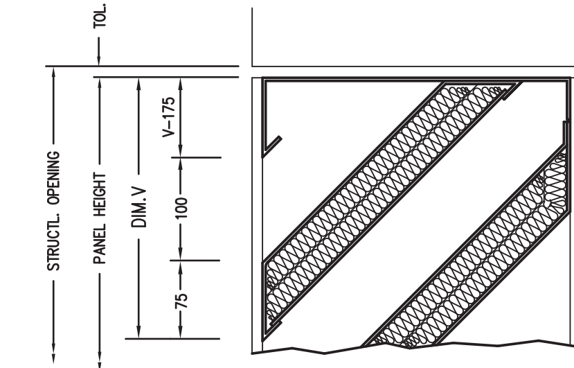
875. HEAD DETAIL
