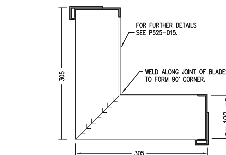
878. 90° EXTERNAL CORNER DETAIL
