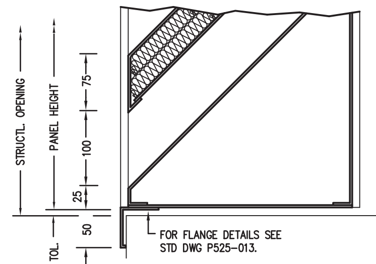
871. CILL DETAIL
