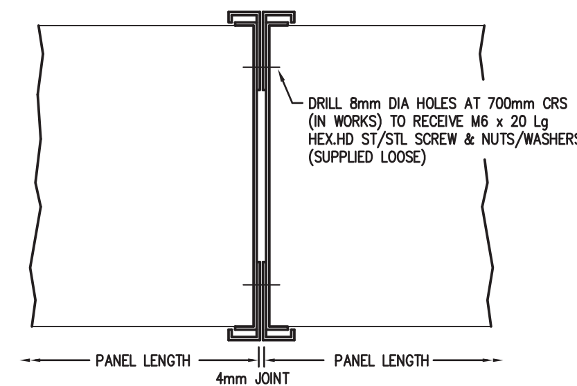
874. HORIZONTAL JOINT DETAIL
